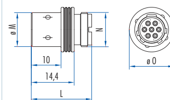
Coupler connector
