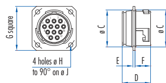
Panel connector
