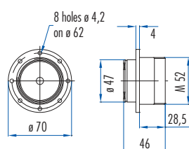
Panel connector
