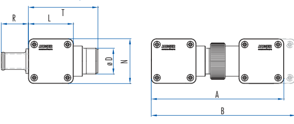
Cable connector and Coupler connector
