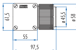
Cable connector
