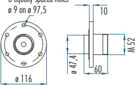
Panel connector
