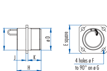
Panel connector
