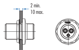
Bulkhead connector
