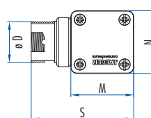
Coupler connector
