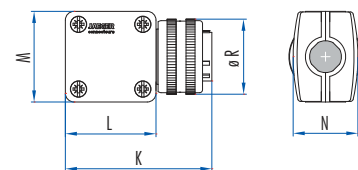
Cable connector
