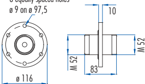
Bulkhead connector
