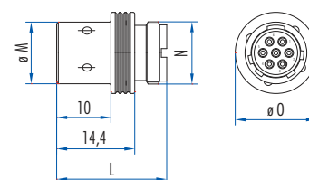
Coupler connector
