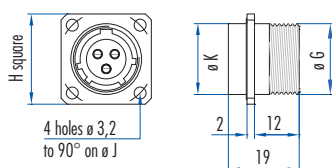
Panel connector
