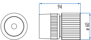
Cable connector
