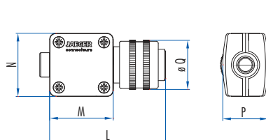
Cable connector
