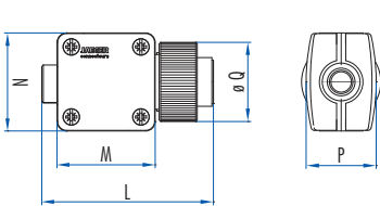
Cable connector
