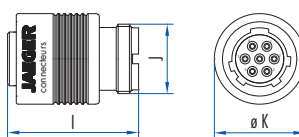
Cable connector
