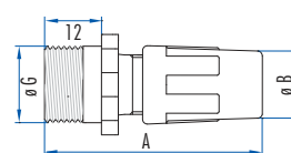
Coupler connector
