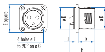
Panel connector
