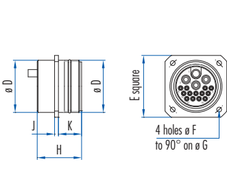
Panel connector
