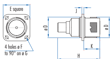
Panel connector
